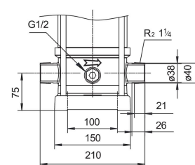
Raccord taraudé (/G)
