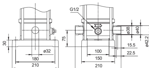
Raccord clamp (/K)
