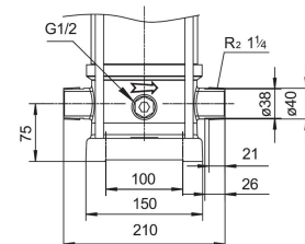
Raccord taraudé (/G)
